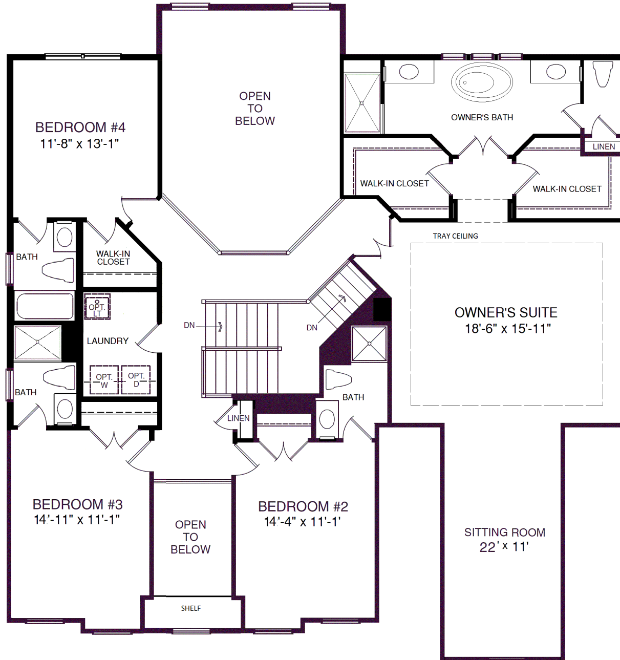
Second Level Floor Plan
